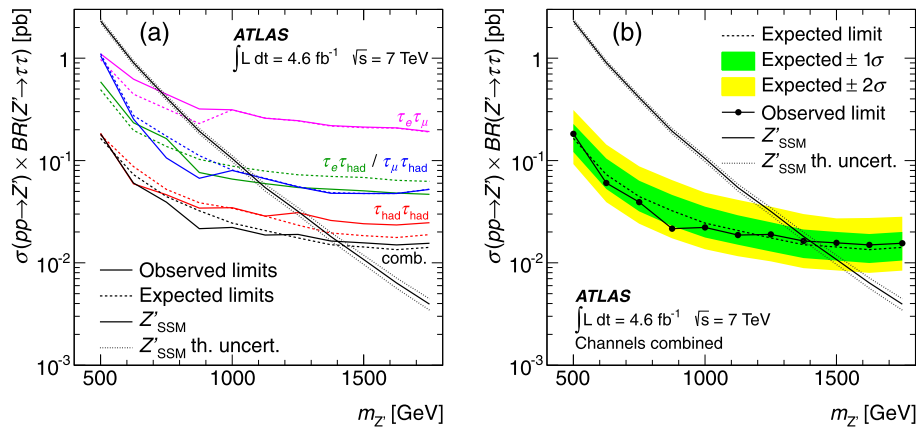
Fig. 2. (a) The expected (dashed) and observed (solid) 95% credibility upper limits on the cross section times \tau^+\tau^- branching fraction, in the \tau_{had}\tau_{had} , \tau_{\mu}\tau_{had} , \tau_e\tau_{had} and \tau_e\tau_{\mu} channels and for the combination. The expected Z'_{SSM} production cross section and its corresponding theoretical uncertainty (dotted) are also included. (b) The expected and observed limits for the combination including 1\sigma and 2\sigma uncertainty bands. Z'_{SSM} masses up to 1.40 TeV are excluded, in agreement with the expected limit of 1.42 TeV in the absence of a signal.
