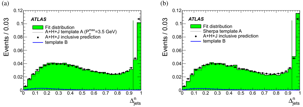
Figure 6. Distribution of \Delta_{\text{jets}}^n in the inclusive A+H+J pseudo-data (dots). (a) A+H+J with p_T^{\text{max}} = 3.5 \text{ GeV} and (b) SHERPA were used to provide Template A. Other details are as in the caption to figure 4.
