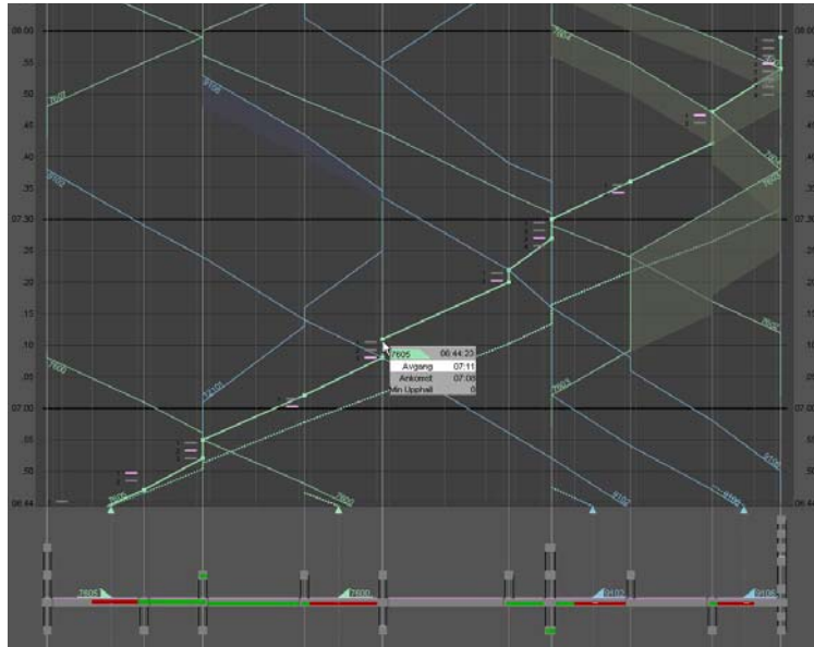
Fig. 4. The re-planning tasks are performed in the graph. A train is selected and highlighted. The selected graph line can be manipulated using the mouse scroll wheel. All re-planning tasks can be performed directly in the interface and the resulting plan is directly visible. Examples of re-planning tasks are changing departure and arrival times, track usage, train speed etc.
