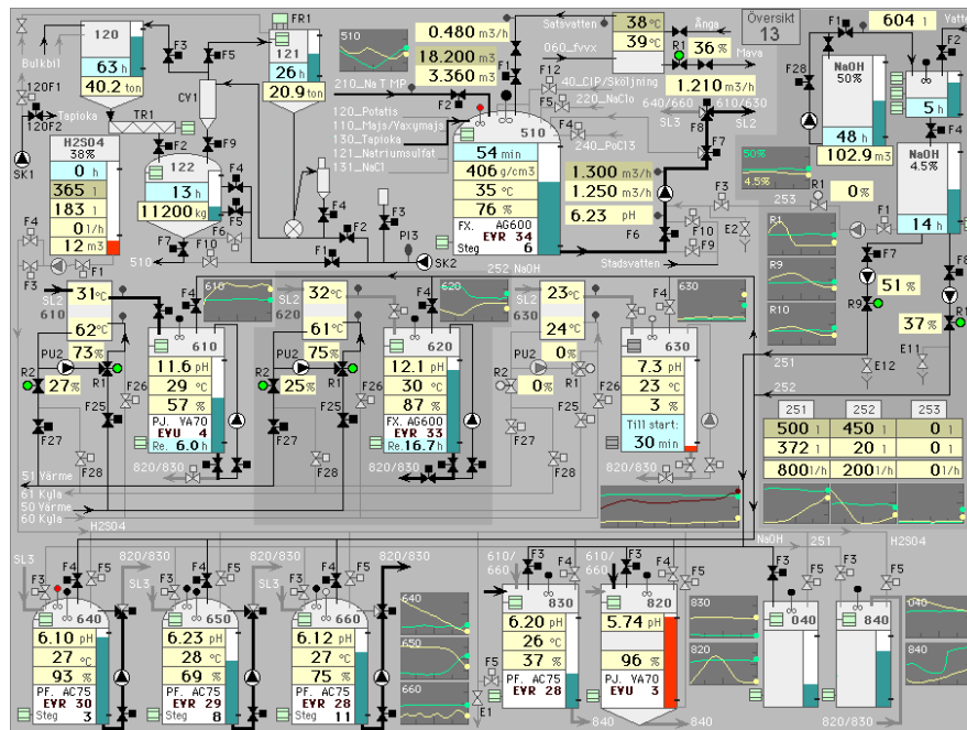
Fig. 8. An example of an operator interface for industrial process control. The visualization contains both static information in the background and dynamic information in the foreground. Information is coded with regard to the importance for the operator. Despite its complexity, for novice users, a skilled operator has no problems to overview and interprets the interface using very low cognitive capacity.
