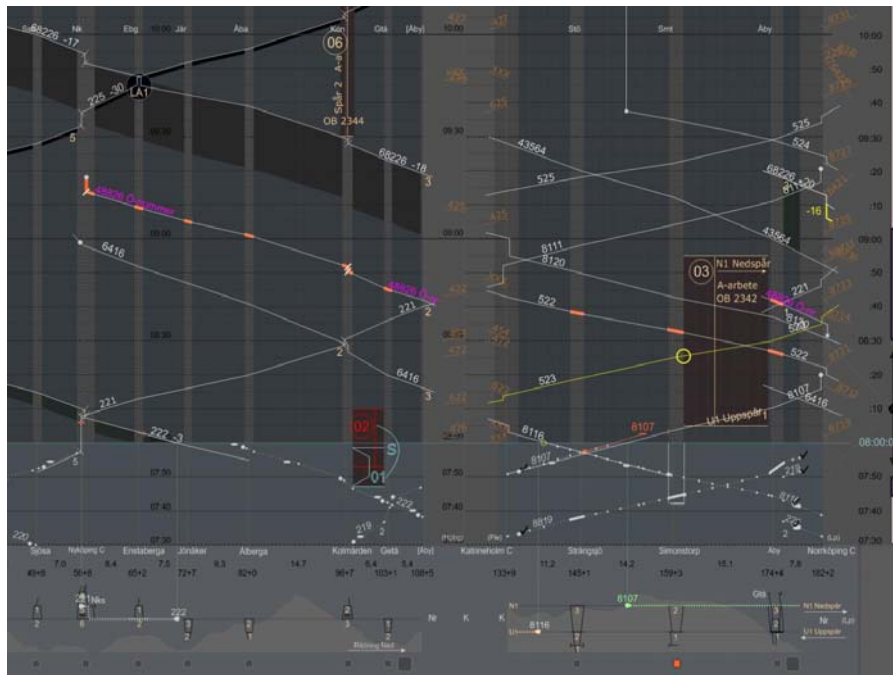
Fig. 3. The new traffic controller user interface. The interface shows the train traffic plan, deviations from the original plan, the planning via in a time-distance graph, the present state (train position and speed), the history, planned maintenance work etc. Static information is e.g. the track structure.
