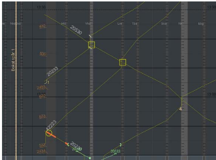
Fig. 5. Example of visualization of conflicts. Conflicts are automatically detected and indicated. Yellow circles here mean a line conflict. A yellow square means station track conflict, i.e. two trains are planned to use the same station track. During re-planning the removal or appearance of a conflict is visualized in real time.
