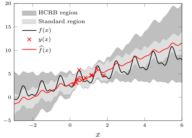
Figure 3: Predictions of f(x) using hyperparameters that have been learned from data. The dark shaded error bars are regions corresponding to f(x) \pm 3\sqrt{\text{HCRB}} .
