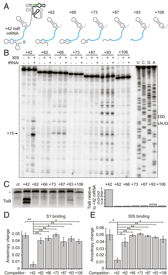
Fig. 5. A 5'-structural element is required for functional standby and tisB mRNA translation. (A) Schematics of the truncated tisB mRNAs. 5' UTR (gray), standby site (blue), ORF (black), and RBS (green). (B) Toeprint assay on the mRNAs as indicated, incubated alone, with 30S, or 30S+tRNA fMet . The toeprint signal (+15 nt) is indicated, as are AUG and SD positions. (C, Left) In vitro translation of +42 tisB mRNA variants in the presence of S 35 -Met. Lane "ct": no mRNA added; asterisk: unspecific label transfer to protein in the extract. See SI Appendix, SI Materials and Methods. (C, Right) Quantitation of band intensities from the gel. The intensity of TisB (+42 mRNA) was set to unity. (D) Competition experiments using 5'-end FAM-labeled +42 tisB mRNA (10 nM) incubated with 80 nM of S1 in the presence or absence of a 50-fold molar excess of the unlabeled mRNAs indicated. (E) Same set-up as in D, but with 30S (150 nM) replacing S1. Anisotropy change calculated from triplicates. *T-test P values < 0.05; **P value < 0.005.
