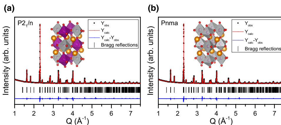
Fig. 1 Refined XRD patterns of \text{Nd}_2\text{NiMnO}_6 using the models a P2_1/n and b Pnma . To visualise the similarities and differences between the two models insets are show for both models
