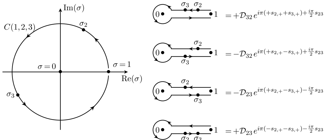
Figure 5. In the \sigma_j = e^{2\pi iz_j} variables, the integration contour \mathcal{C}(1,2,3) is the unit circle in the left panel, where the phases of \sigma_2 and \sigma_3 are ordered according to z_2 < z_3 . Similar to figure 4, we replace \mathcal{C}(1,2,3) by the homotopy-equivalent combination of paths visualized in the right panel. For each of the four inequivalent relative positions of \sigma_2 and \sigma_3 , the Koba-Nielsen factor (5.2) introduces a different phase that depends on s_{2+} , s_{3+} and s_{23} .
