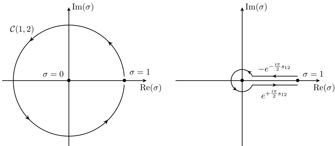
Figure 4. As depicted in the left panel, the integration contour \mathcal{C}(1, 2) in the \sigma_2 = e^{2\pi iz_2} variable is the unit circle |\sigma_2| = 1 . When replacing \mathcal{C}(1, 2) by the homotopy-equivalent combination of paths visualized the right panel, the multivalued part of the integrand \sigma_2^{s_{12}/2} introduces phases e^{\pm \frac{i\pi}{2} s_{12}} depending on the sign of the small imaginary part of \sigma_2 .
