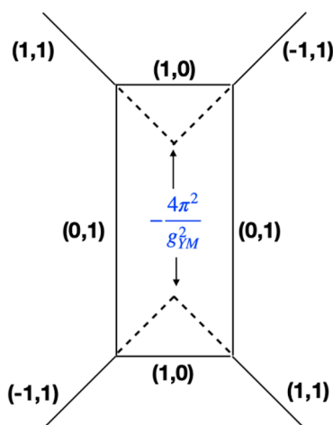
(b) g_{\text{YM}}^2 < 0
