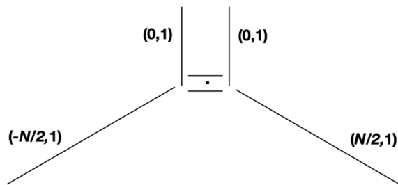
Figure 3. (p, q) web for \mathcal{N} = 1 SU(N/2) gauge theory with a Chern-Simons term at level k = N/2 .
