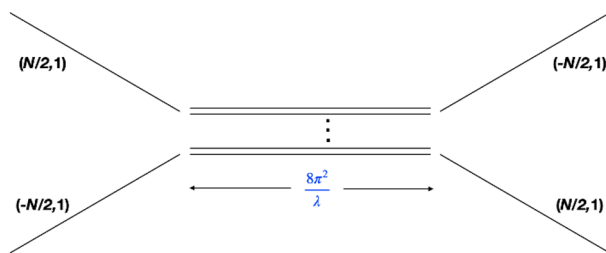
(a) g_{\text{YM}}^2 > 0
