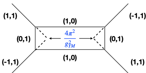
(a) g_{\text{YM}}^2 > 0
