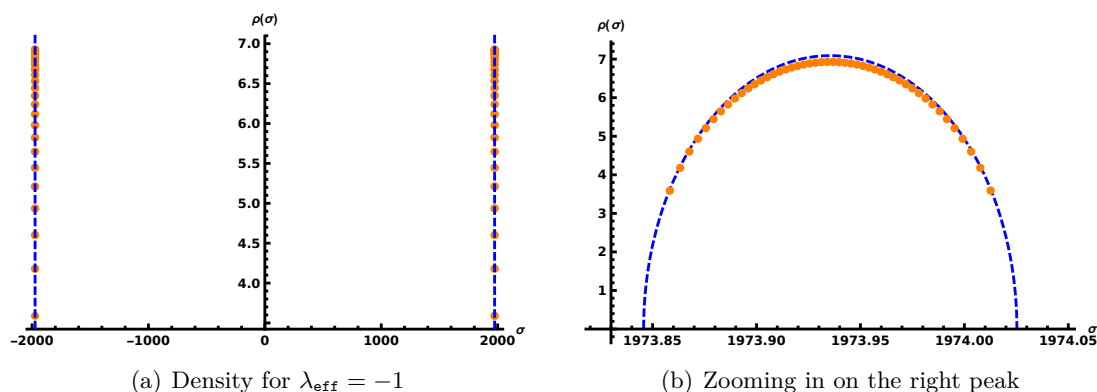
Figure 8. Eigenvalue density \rho(\delta\sigma) for \lambda_{\text{eff}} = -1 , N = 50 and N_f = 4 . The dashed lines represent the analytical solutions (6.6) and (6.17).
