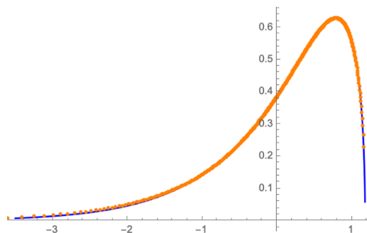
Figure 6. Eigenvalue density for SU(N/2)_{N/2} Chern-Simons theory with N/2 = 500 . The orange dots are the numerical result while the blue curve is a fit to the function a\sqrt{b - \sigma} e^{c\sigma} with a best fit at a = 0.3566 , b = 1.182 and c = 1.308 .
