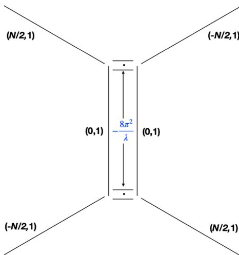
(b) g_{\text{YM}}^2 < 0
