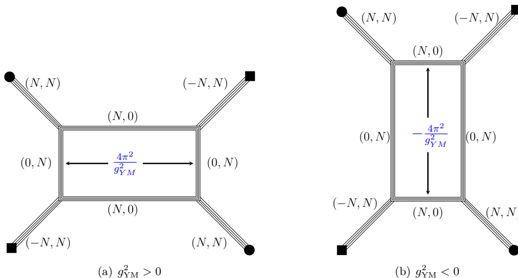
Figure 11. (p, q) web for a \text{USp}(2N) gauge theory with a hypermultiplet in the antisymmetric representation at positive and negative coupling.
