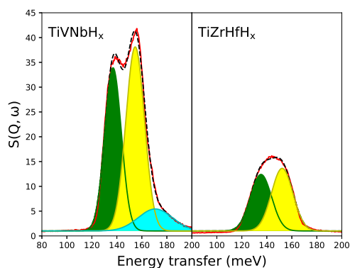
Fig. 4. Gaussian fits to the experimental INS spectra of \text{TiVNbH}_x (left) and \text{TiZrHfH}_x .
