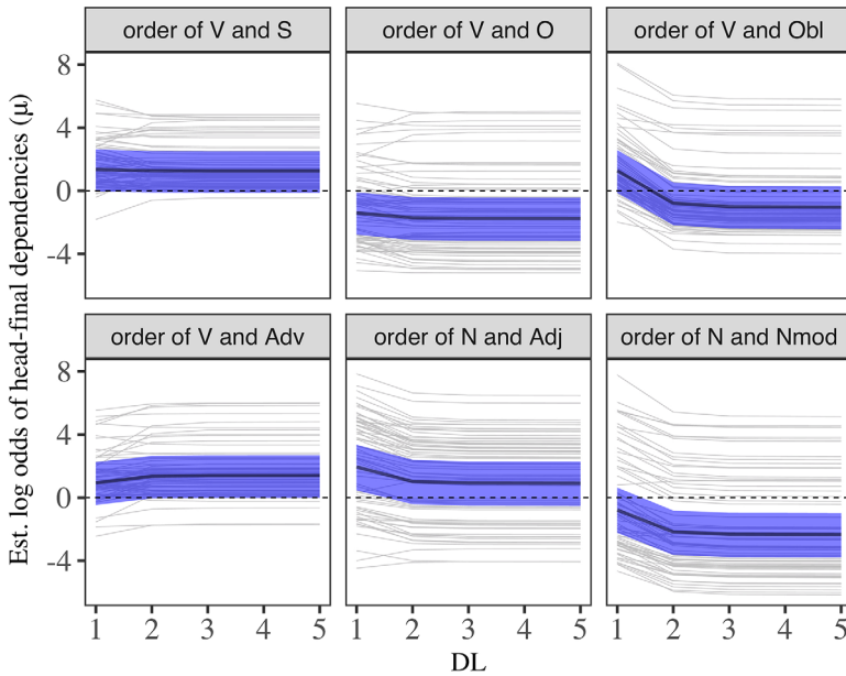
Fig. 3. Monotonic effect of DL on word order directions ( \mu in log odds) across dependency types, after conditioning on the language-specific effects (“random slopes”) and the overall variation between families and areas (“random intercepts”). Higher \mu values indicate higher (log) odds of HF orders. The thick black lines show the estimated mean effect of DL at the population level (“fixed effects”), and the thin gray lines show the estimated mean effects in individual languages (“random effects”). The colored ribbons indicate 90% credible intervals around the population-level mean.
