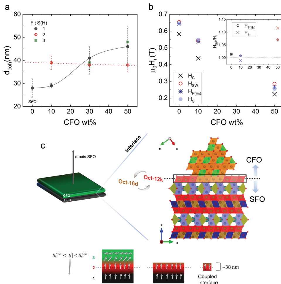
Figure 6. a) Coherent sizes d_{\text{coh}} (indices 1-2-3 refer to magnetic components extracted from the fitting); the red dashed line is a linear fitting (with a nearly zero slope) for the critical thickness of the CFO phase. b) Summary of all the field parameters H_C , H_{\text{SW}} , H_S , H_{\text{P}(H_C)} , from the experimental measurements. In the inset, ratios between H_{\text{SW}} (from SFD) and H:H_S (from viscosity) and H_{\text{P}(H_C)} (from FORC projections along H_C ) are shown; c) SFO/CFO interface with the crystallographic orientation, and sketch of the magnetic reversal mechanism when the CFO fraction increases.
