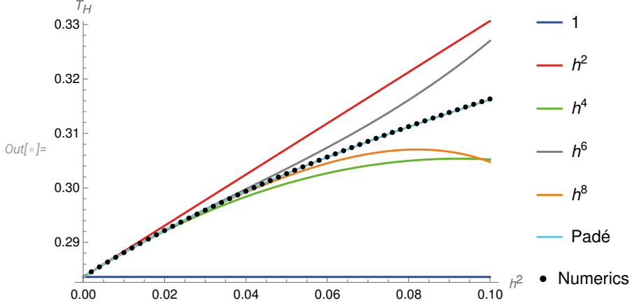
Figure 9.2. The perturbative solution of the quantum spectral curve truncated to various orders is compared to the numerical solution in the range 0 \leq h^2 \leq 0.1 and the [4/4] Padé approximation (9.57). Figure taken from Paper VII.
