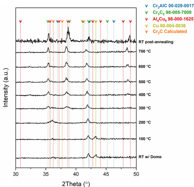
Fig. 1 XRD patterns obtained during, and after, in situ XRD annealing of as-deposited \text{Cr}_2\text{AlC}/\text{Cu} assemblies, up to 700 °C with 100 °C steps.
