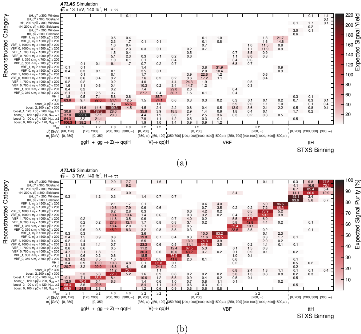
Figure 1. (a) Expected SM H \rightarrow \tau\tau signal yield and (b) expected signal purity in each signal region of the analysis ( y -axis). Yields are summed over the three \tau\tau channels ( \tau_e\tau_\mu , \tau_{lep}\tau_{had} , \tau_{had}\tau_{had} ). Only entries with a value above 0.1 are shown in the plots.
