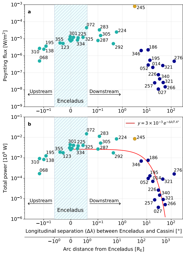
Figure 5. (a) Poynting fluxes ( S ) and (b) total powers measured locally for large-scale perturbations ( <0.1 Hz), as a function of the moon-spacecraft longitudinal separation \Delta\lambda and arc distance from Enceladus. The red line in panel (b) represents a least square fit of an exponential function.
