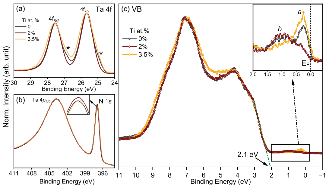
FIGURE 2 | (a) Ta 4f, (b) N 1s core-level hard X-ray photoelectron spectra with an inset shows zoomed view of undoped, 2 and 3.5 at% Ti-doped \text{Ta}_3\text{N}_5 thin films. (c) Valance band spectra measured using hard X-rays of undoped, 2 and 3.5 at% Ti-doped \text{Ta}_3\text{N}_5 thin films. Inset shows zoomed view near Fermi-Level.
