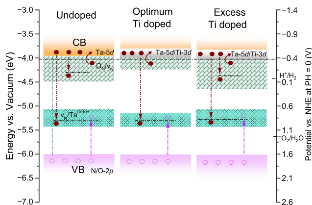
FIGURE 6 | Schematic band diagram of undoped \text{Ta}_3\text{N}_5 , optimum Ti-doped, and excess Ti-doped \text{Ta}_3\text{N}_5 .
