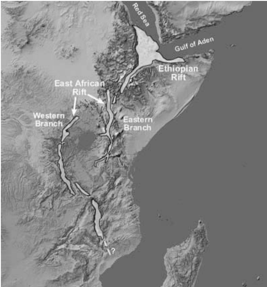
Figure 1. Map of the Eastern and Southern Africa region with the nine countries that are participating in the ESARSWG seismological network. The East Africa rift system extends from Eritrea / Ethiopia in the north through Uganda, Kenya, and Tanzania to Malawi, Zambia, Mozambique, and Zimbabwe in the extreme south. In East Africa, the rift splits into two branches – the Eastern and Western branches. In Zimbabwe and Southern Mozambique, the rift is ill defined, and incipient rifting is identified by earthquake activity. Earthquakes of magnitude in excess of 6.0 have occurred along and over the entirety of the region from the south in Mozambique to Ethiopia in the north.
