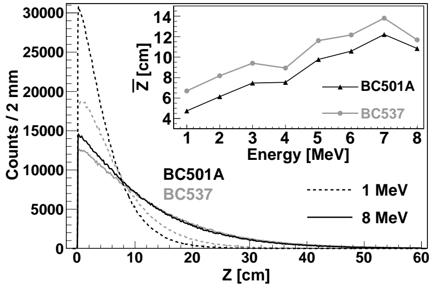
Figure 7: Distributions of the depth of the significant interaction ( Z ) for two neutron energies and two scintillators, BC501A and BC537. The type of the scintillator is marked with black and grey lines for BC501A and BC537, respectively. The line pattern marks the neutron energy as shown in the legend. A total of 10^6 neutrons were simulated in each case. The insert shows the dependence of the mean significant interaction depth ( \bar{Z} ) on the neutron energy. Lines connecting the points in the insert are drawn only to guide an eye.
