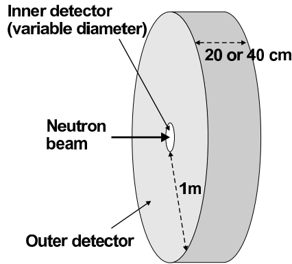
Figure 9: Setup used in the evaluation of the probability that one neutron generates a signal in more than one detector module.
