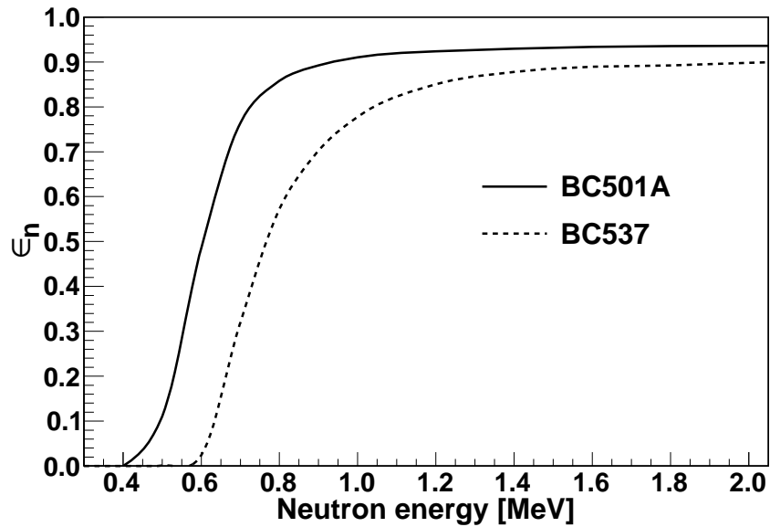
Figure 15: Neutron detection efficiency as a function of neutron energy for the two scintillators BC501A and BC537. The detector had a diameter of 50 cm and was 60 cm long.
