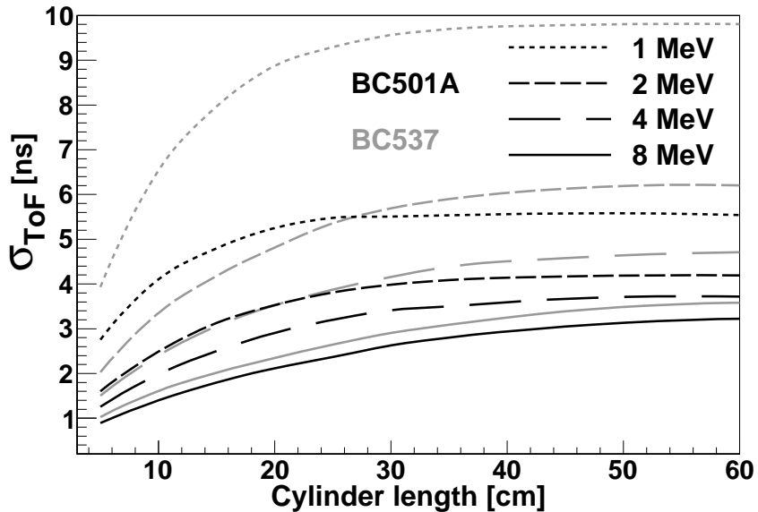
Figure 11: Width (one standard deviation) of the time-of-flight distributions as a function of the cylinder length for BC501A (black lines) and BC537 (grey lines), and for 1, 2, 4 and 8 MeV neutrons.
