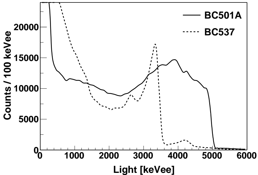
Figure 2: Geant4 simulation: scintillator light output for 10 MeV neutrons in the detector of Fig. 1. An instrumental response function was not included in this calculation.
