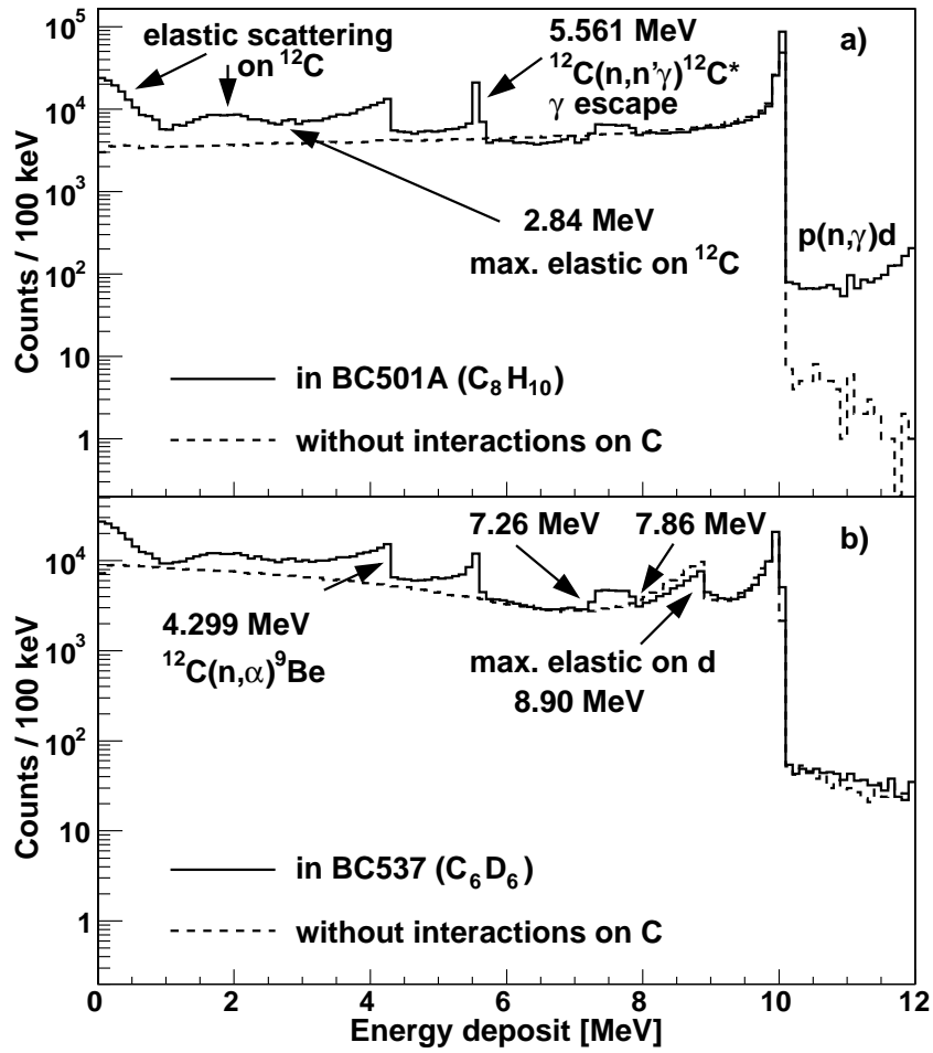
Figure 1: Geant4 simulation of the energy deposited by 10 MeV neutrons in the two liquid scintillators (a) BC501A ( C_8H_{10} ) and (b) BC537 ( C_6D_6 ). The detectors have a diameter of 12.7 cm (5 inch) and a length of 20 cm. The detector walls were not included in the simulations. The energy-deposit spectra for the hypothetical detector material consisting only of protons and deuterons (without carbon) are drawn with dashed lines.
