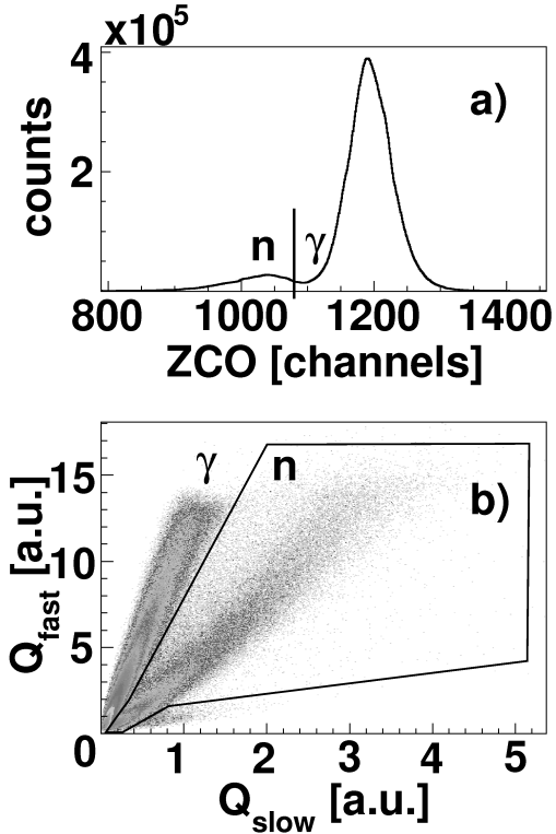
Figure 4: Zero-cross-over time (ZCO) histogram (a) and two dimensional charge comparison plot (b) used for the neutron- \gamma discrimination in the Uppsala and Warsaw measurements, respectively. See text for the definition of Q_{fast} and Q_{slow} .
