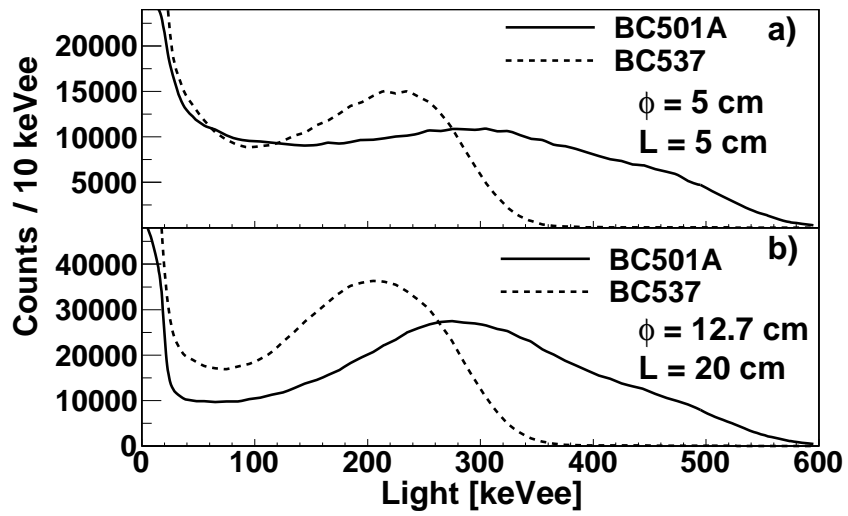
Figure 14: Light produced by a pencil beam of 2 MeV neutrons in two cylindrical BC501A and BC537 detectors of different size: a) a small and b) a large detector. The dimensions of the detectors are shown in the legends.
