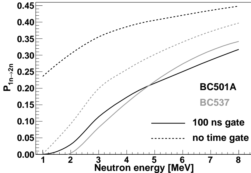
Figure 13: Influence of the 100 ns detection time limit on the P_{1n \rightarrow 2n} probability.
