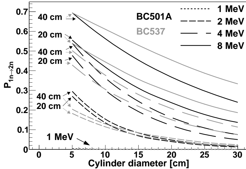
Figure 10: The probability to have an interaction in two detector modules ( P_{1n \rightarrow 2n} ) as a function of the cylinder diameter. Four sets of lines, corresponding to neutron energies 1, 2, 4 and 8 MeV, are shown for each of the two scintillators, BC501A and BC537 in black and grey, respectively. Cylinders with two lengths, 20 and 40 cm, were used and the respective lines are marked with text labels and arrows.
