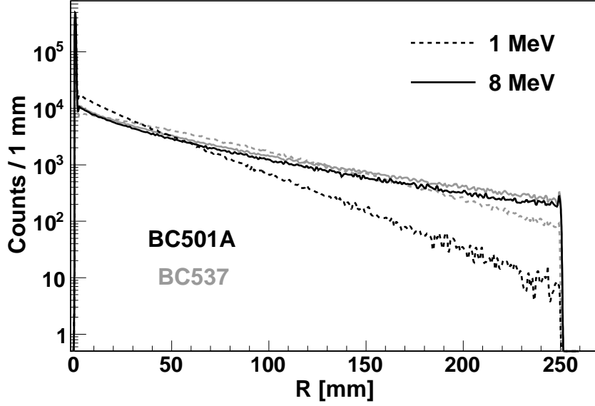
Figure 8: Distribution of the distance ( R ) between the position of the first significant interaction and the axis of the incoming neutrons. The results of the simulations for two neutron energies (1 and 8 MeV) are shown with black and grey lines for the two scintillators, BC501A and BC537, respectively. A pencil beam of 10^6 neutrons were shot into the centre of the cylindrical detector in each of the presented cases.
