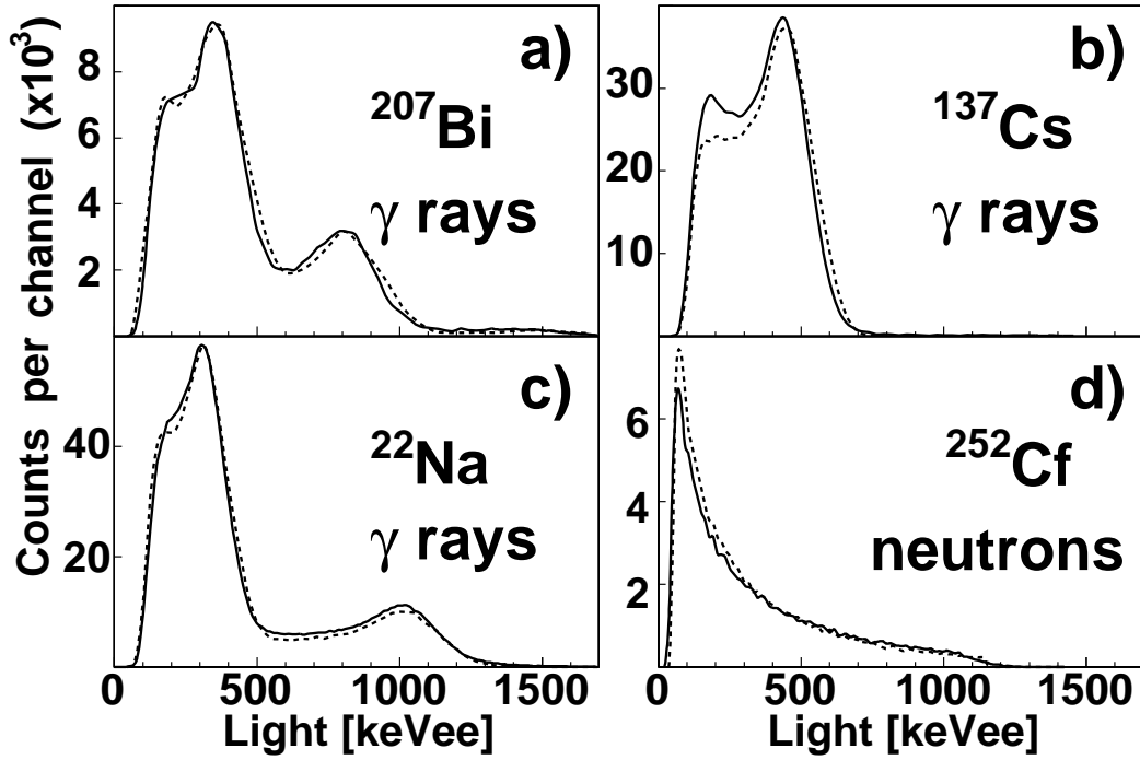
Figure 5: Experimental (solid) and simulated (dotted line) \gamma -ray spectra for the NORD-BALL detector (a-c) and a neutron spectrum for the cylindrical detector (d). The simulated \gamma -ray spectra shown in plots (a) and (c) are normalised to the maximum of the experimental distributions, while the 137 Cs \gamma -ray and 252 Cf neutron histograms show true measured and simulated numbers of counts, corresponding to the source activity. The 207 Bi and 22 Na sources were placed at a distance of 20 cm from the front of the detector, while for 137 Cs and 252 Cf this distance was 50 and 5 cm, respectively.
