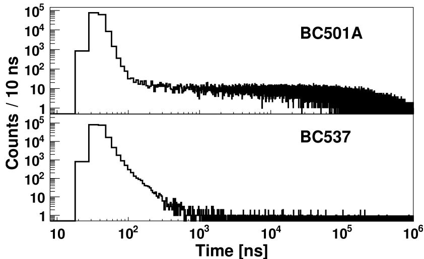
Figure 12: Times of the significant interaction in the outer detector of the two scintillators shown in Fig. 9. A source of 2 MeV neutrons was placed 51 cm in front of the detectors and the time measurement starts when a neutron is emitted from the source. The detectors were 20 cm long and the diameter of the inner detector was 12.7 cm.
