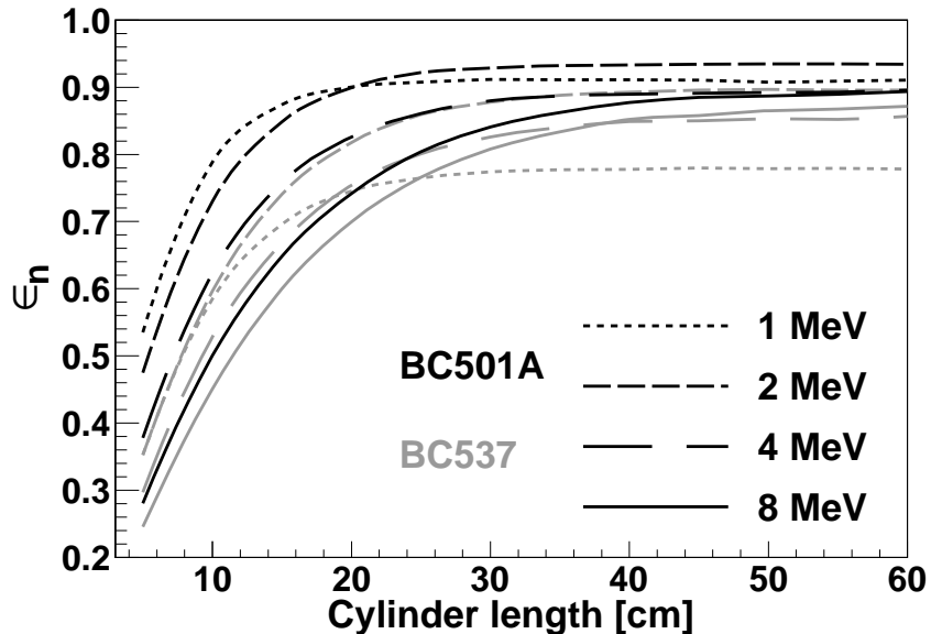
Figure 6: Neutron detection efficiency ( \epsilon_n ) as a function of the cylinder length for the two scintillators BC501A (black lines) and BC537 (grey lines) and for 1, 2, 4 and 8 MeV neutrons.
