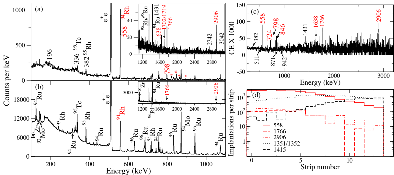
FIG. 1: (Color online) Gamma-ray spectra associated with the decay of (a) the ^{94}\text{Pd} nuclei, where symbols are used to mark 822, 846 and 896 (*) and 863 keV (+) lines and (b) all of the nuclei implanted in the “active DSSSD”. The majority of the lines can be associated with the known decays of nuclei as indicated [35]. New as well as the known \gamma transitions in ^{94}\text{Rh} are marked in red. Unidentified peaks are marked in black only with their energies. (c) The correlation efficiencies, CE, (multiplied by 1000) deduced from the spectra in (a) and (b). (d) Implantsations per strip in the “active DSSSD” (i.e. hit distributions) corresponding to several \gamma rays are also shown. See the text for details.
