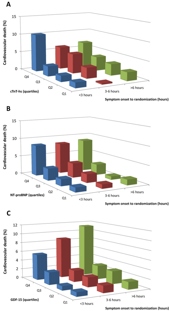
Occurrence of CVD for quartiles of cTnT-hs (A), quartiles of NT-proBNP (B), and quartiles of GDF-15 (C) stratified according to time between onset of symptoms and randomization.
