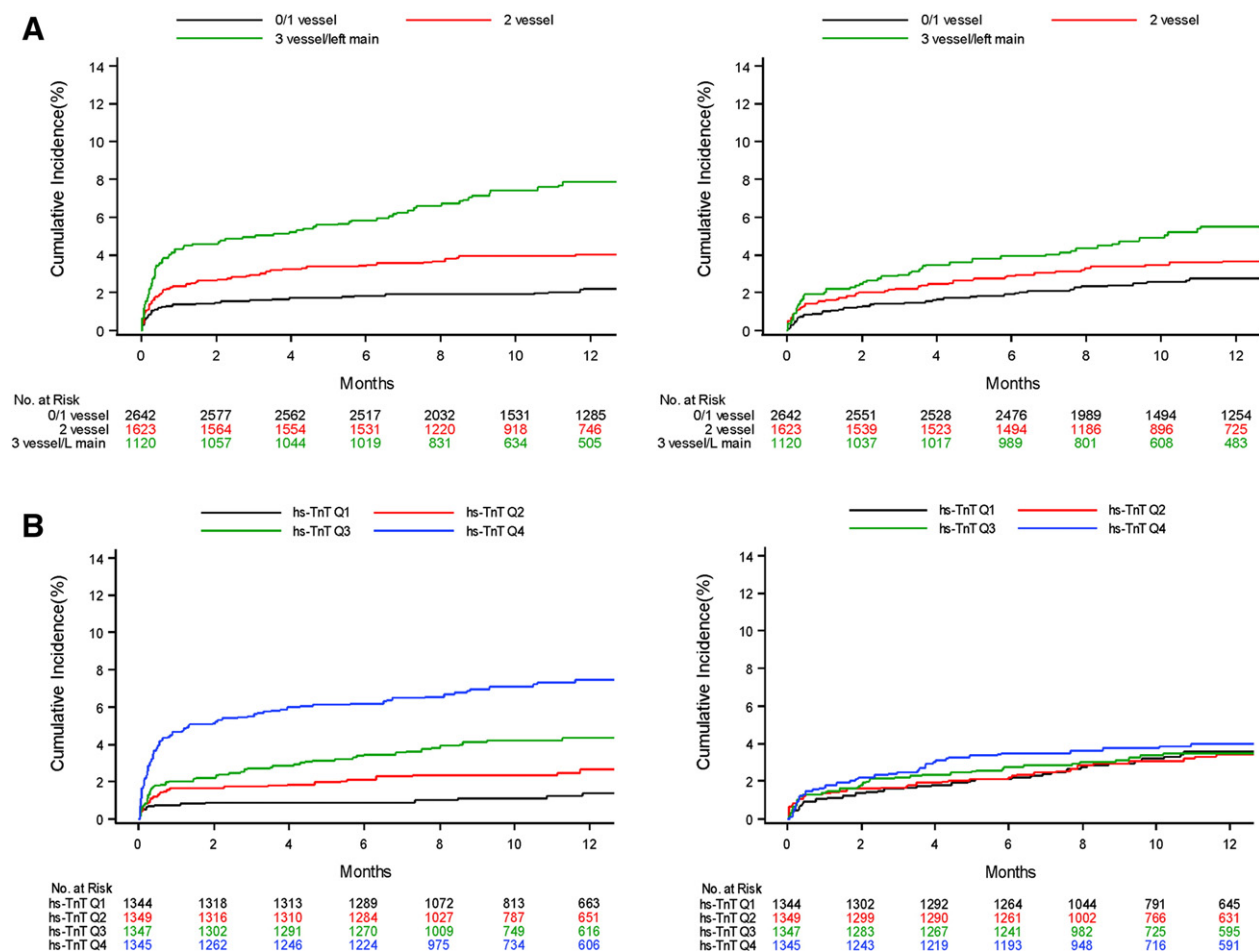
Occurrence of CVD (left side of figure) and spontaneous MI (right side of figure) according to extent of CAD (A) and quartiles of cTnT-hs (B).
